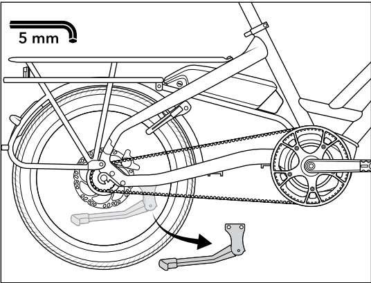
1. Remove the existing kickstand.
