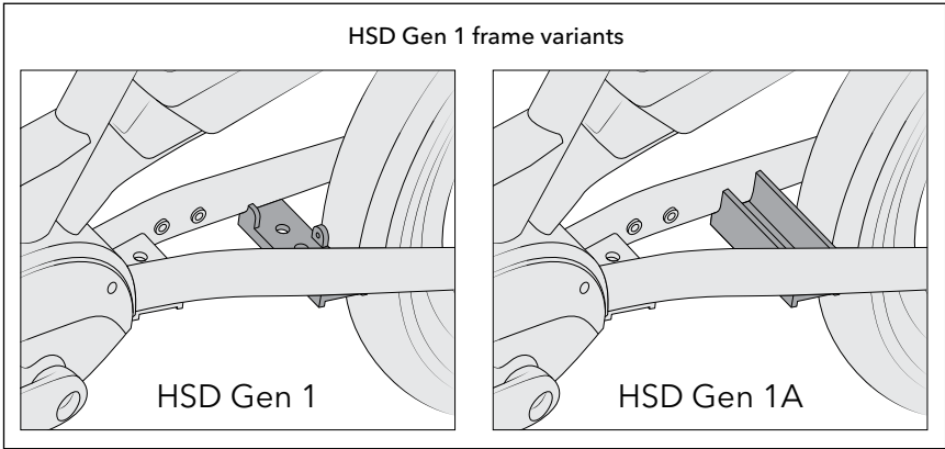
2. Identify the HSD frame variant by locating the kickstand mount in front of the rear wheel.
